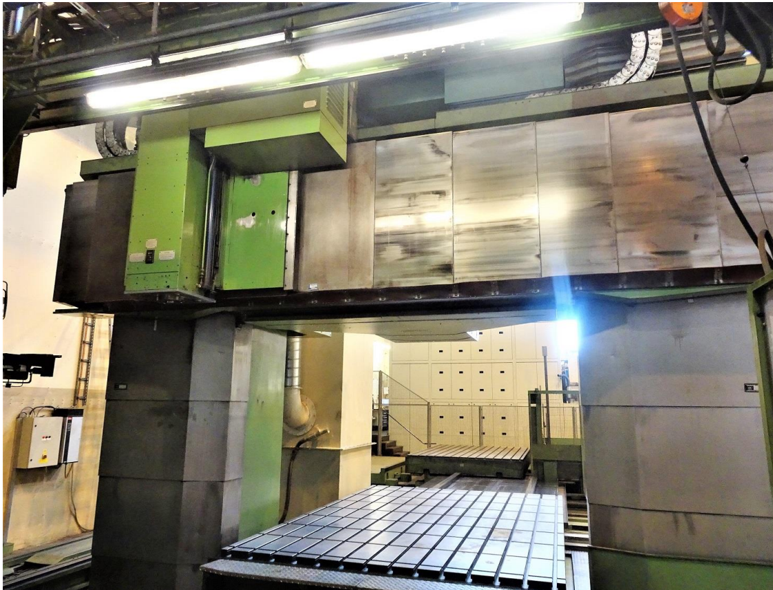
machine at production place company Gebr. HELLER/Nürtingen
